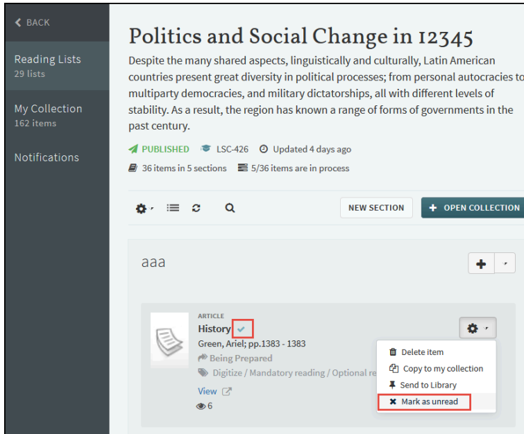
Reading List Page - Mark as Unread
